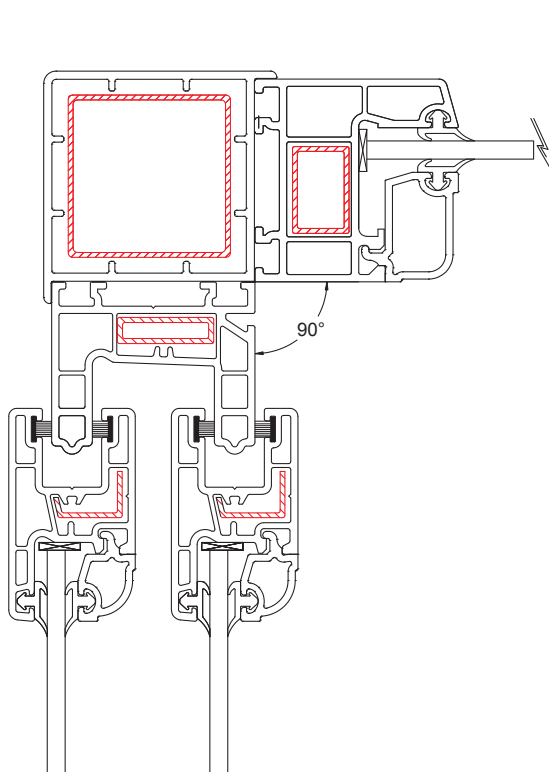
CORNER ASSEMBLY 90°
