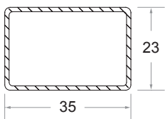
'Z' Mullion Code No : ST - 753
