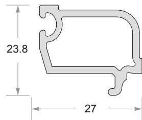
Single Glazing Bead Code No : DP - 554
