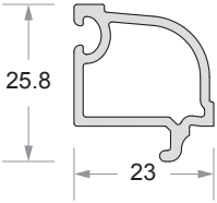
Double Glazing Bead ( 24mm ) Code No : DP - 755
