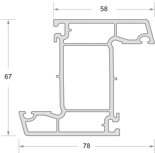
'Z' Mullion Code No : DP - 753
