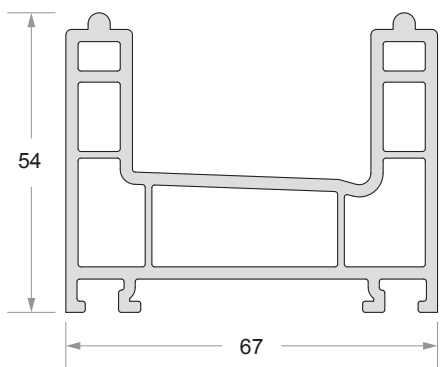
2 Track Sliding Frame Code No : DP - 701
