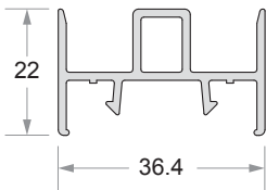
Sash Joint Code No : DP - 508
