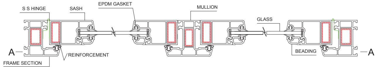
Casement Window With T Profile
