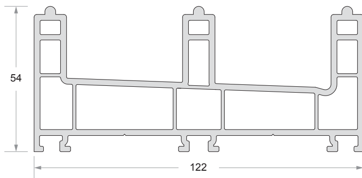
3 Track Sliding Frame Code No : DP - 702
