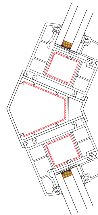
CORNER ASSEMBLY 135°
