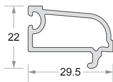
Single Glazing Bead ( 4-6mm ) Code No : DP - 707
