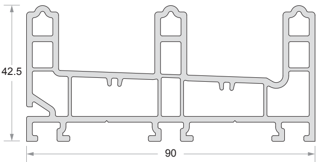
3 Track Sliding Frame Code No : DP - 502
