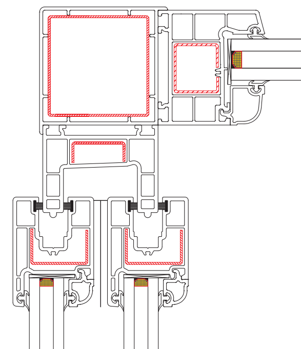
CORNER ASSEMBLY 90°
