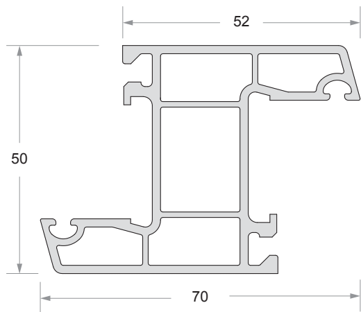
'Z' Mullion Code No : DP - 553
