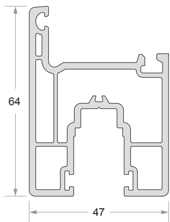
Sliding Window Sash Code No : DP - 703
