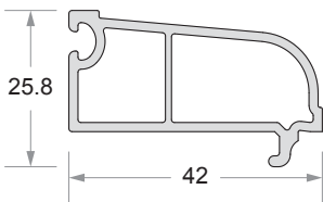
Single Glazing Bead ( 4 - 6mm ) Code No : DP - 754
