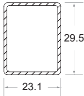
False Mullion Code No : ST - 757
