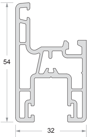
Sliding Window Sash Code No : DP - 503
