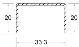
Window Sash Code No : ST - 703
