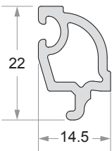
Single Glazing Bead Code No : DP - 507
