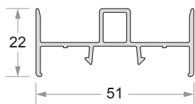
Sash Joint Code No : DP - 708
