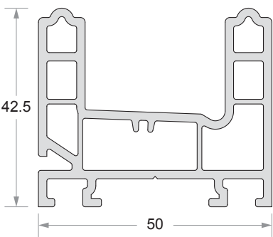
2 Track Sliding Frame Code No : DP - 501
