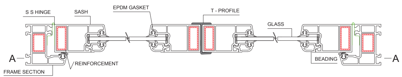
Casement Window With T Profile
