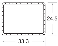
Sash / Mullion Code No : ST - 752
