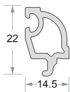
Double Glazing Bead ( 20mm ) Code No : DP - 507
