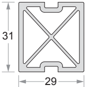
Reinforcement Code No : DPDR - 3129
