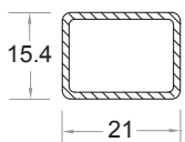
'Z' Mullion Code No : ST - 553
